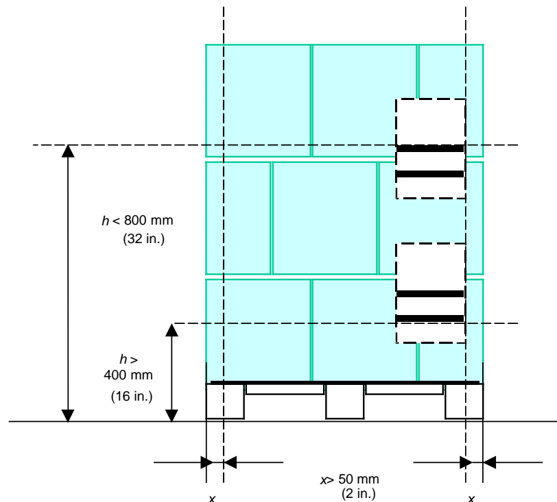
Figure 6.8.1.1 – 1. Symbol placement on pallets
